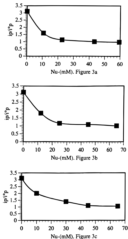
Figure 3. Analysis of the cyclic voltammetric peak current of the redox-catalyzed electrochemical induction of the substitution of n\text{-C}_4\text{F}_9\text{I} (6 mM) by 19^- (a), 14^- (b), and 15^- (c). Mediator: nitrobenzene (2 mM); scan rate = 0.2 V/s; DMSO + 0.1 M \text{Et}_4\text{NBF}_4 at 25 °C.
